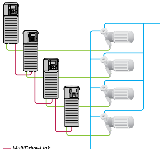
Example of connection with MD-Link
