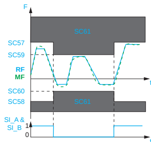
Activation of the SMS function
