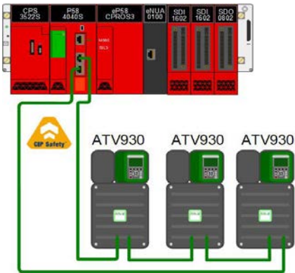
Example of CIP Safety architecture with ATV930 drives
