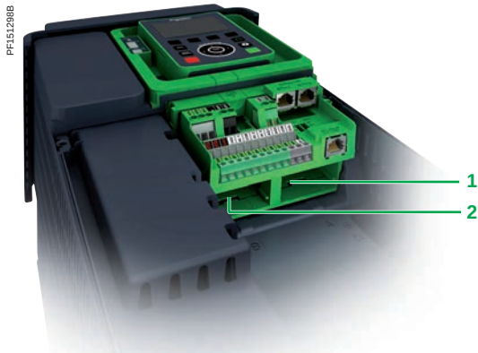
Altivar Process drives slots for additional I/O modules
