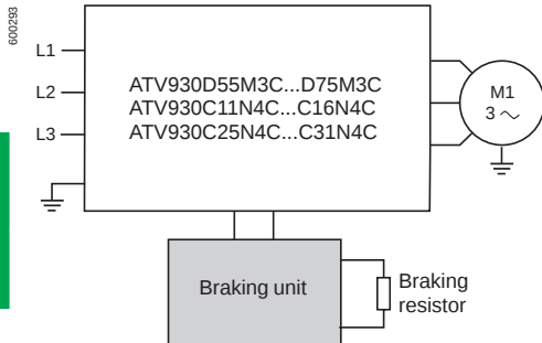
Altivar Process drive with braking unit
