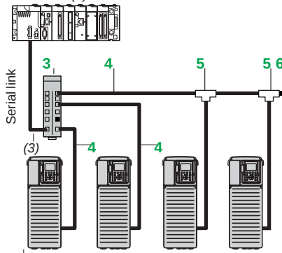
Example of serial link architecture
