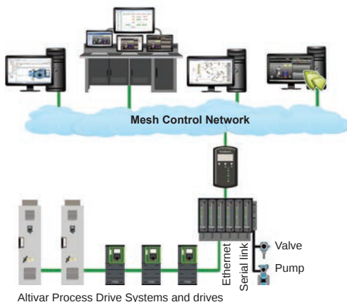
Altivar Process in EcoStruxure Foxboro DCS architecture
