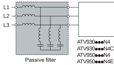
Altivar Process drive with passive filter
