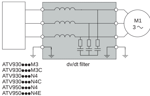
Altivar Process drive with dv/dt filter
